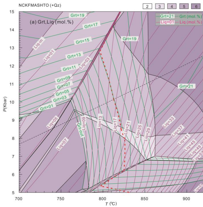
Fig. S2. (a-e) P - T pseudosections of Fig.6, contoured for the mode of garnet (Grt), liquid/melt (Liq), biotite (Bt), K-feldspar (Kfs), plagioclase (Pl) and Aluminosilicate (Als): Ky/Sil, for compositional isopleths of garnet ( X_{Grs} and X_{Prp} ), X_{Mg} of biotite and X_{An} in plagioclase. The red dashed line presented here represents the solidus calculated from measured bulk composition for reference.
